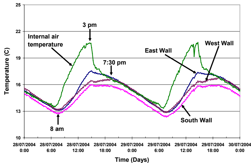
Figure 5. Surface temperature for the interior walls, 28 and 29 July 2004
