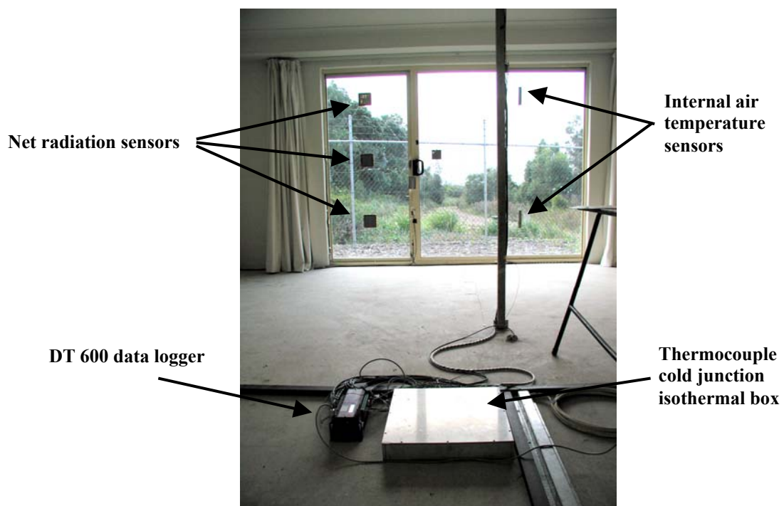
Figure 2. Internal view of Module 3
