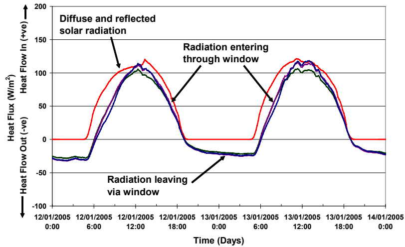
Figure 7. Heat exchange via window, slab and interior walls 12 and 13 January 2005
