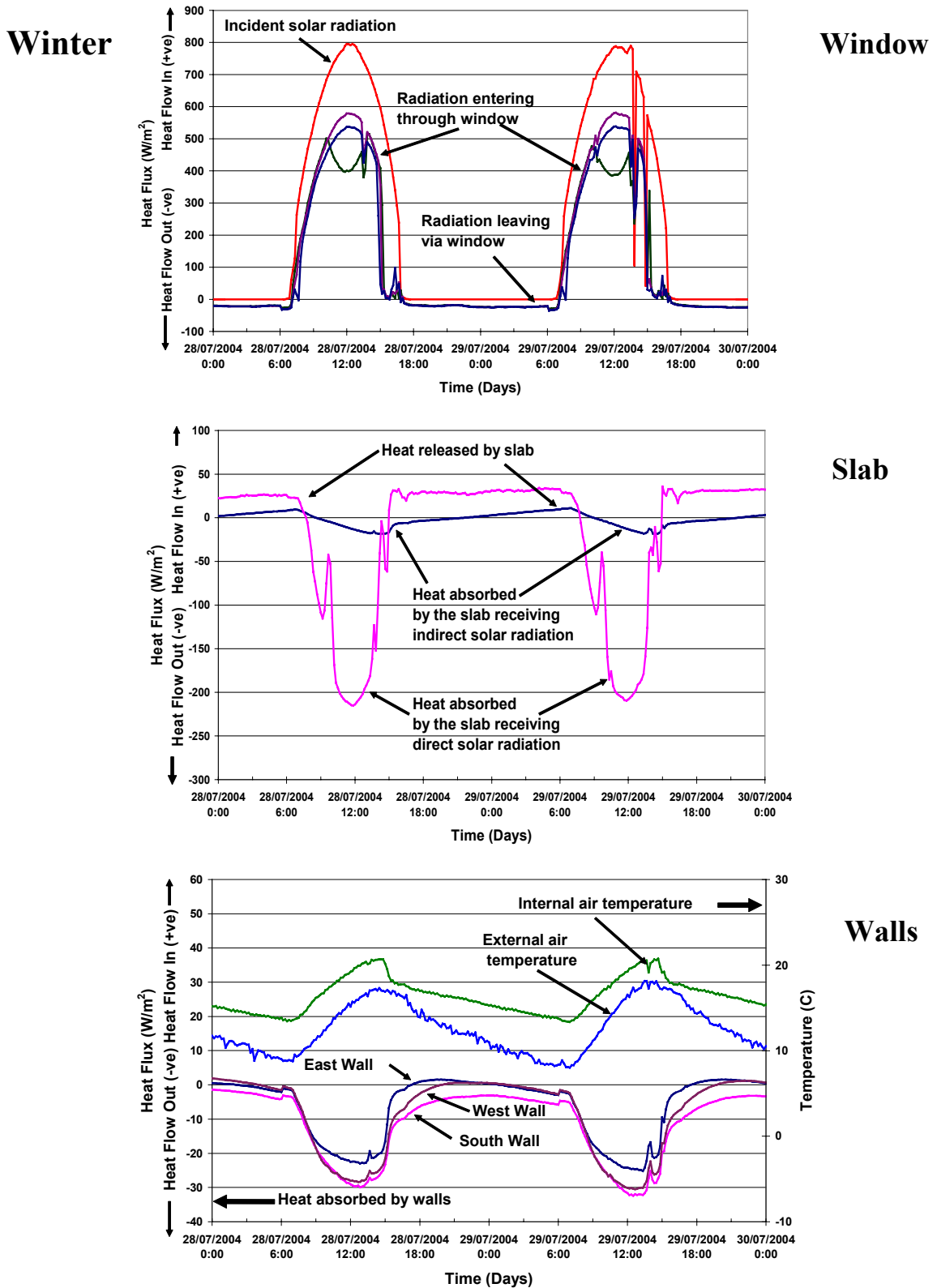
Figure 4. Heat exchange via window, slab and interior walls, 28 and 29 July 2004
